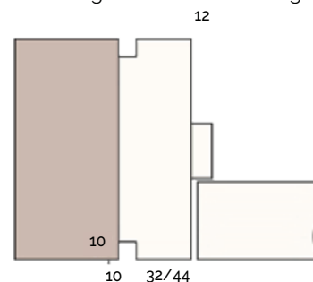
Plain lining frame with shadow gap detail
