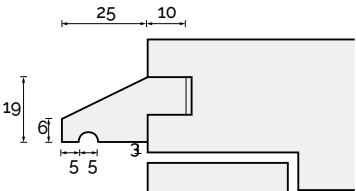
Frame head drip
