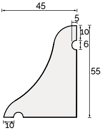
Standard weatherboard
