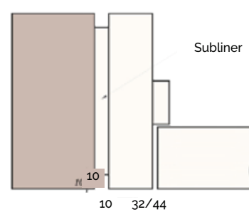
Plain lining frame with hardwood subliner
