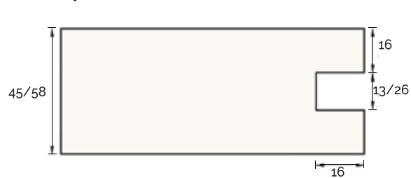
Square Shoulder
