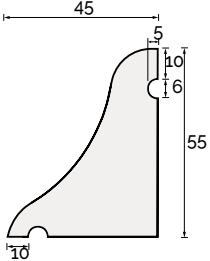
Standard weatherboard
