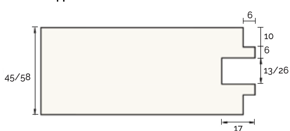
Stepped Rebate
